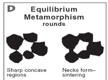
Strong bonds form between grains
