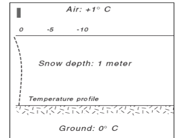
A typical spring snow temperature profile
