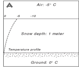
A small temperature gradient promotes equilibrium metamorphism
