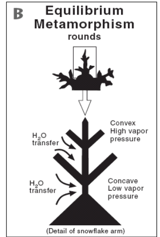
Original crystals lose their sharp points
