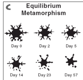
Rounds develop from equilibrium metamorphism
