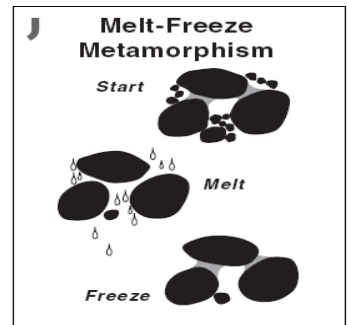
The melt-freeze cycle
