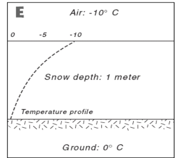
A large temperature gradient promotes kinetic metamorphism
